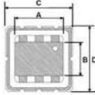
SAW Filter Package
