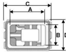
Oscillator (OSC) Package
